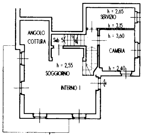
PIANO TERRENO
